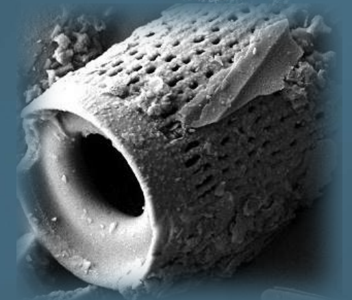
Scanning electron microscope image of Diafiltra® particle. Image size 20µm x 15µm.
